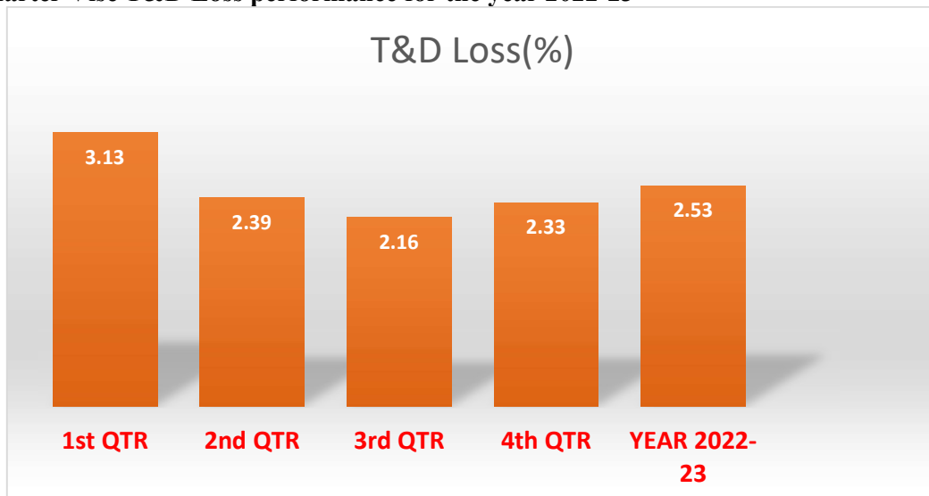
Quarter Wise T&D Loss performance for the year 2022-23
